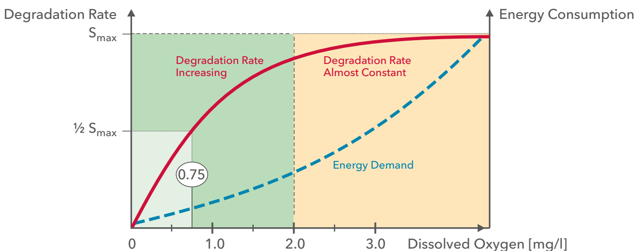
NH 4 -N degradation rate vs. D.O. concentration
